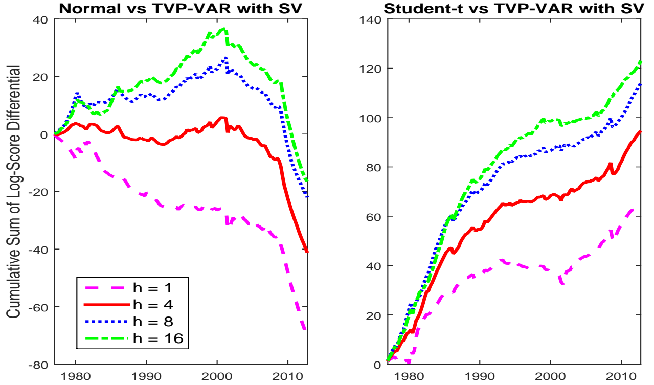
Figure 6: Cumulative sum of the logarithm score over time: comparison with a TVP-VAR with stochastic volatility. A rising line suggests that the adaptive AR(1) model with Gaussian (left panel) and Student-t innovations (right panel) outperforms the TVP-VAR with stochastic volatility.
